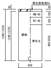
③④配水管撤去VPφ75(100) DP: 1200
